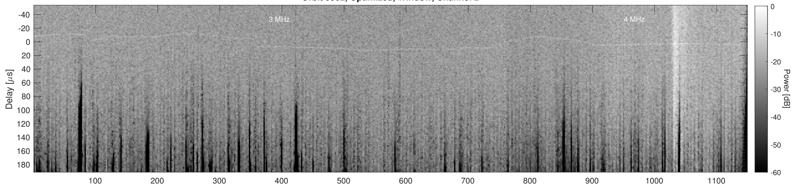
Orbit 9902, Cluttergram
