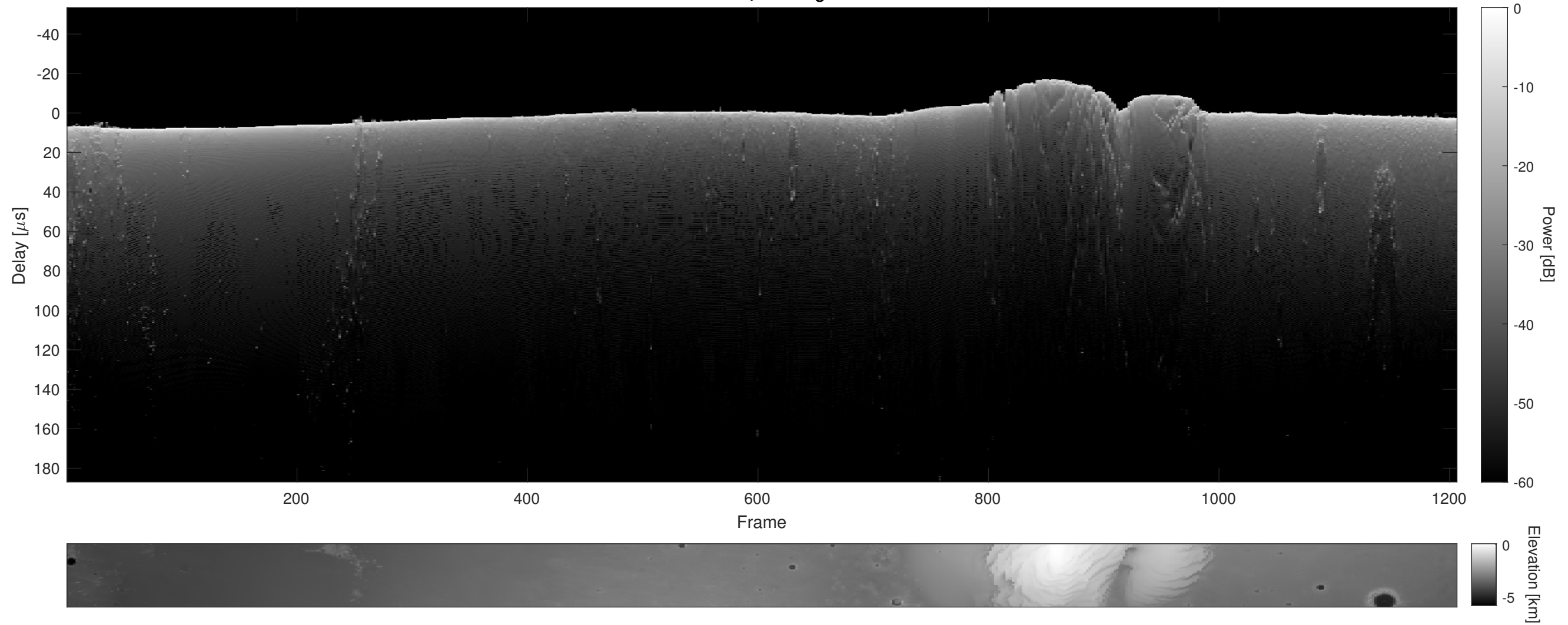
Orbit 9903, Cluttergram
