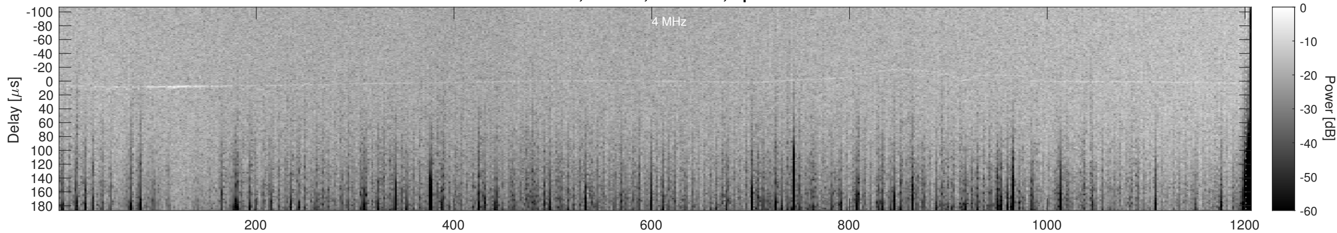
Orbit 9903, Cluttergram
