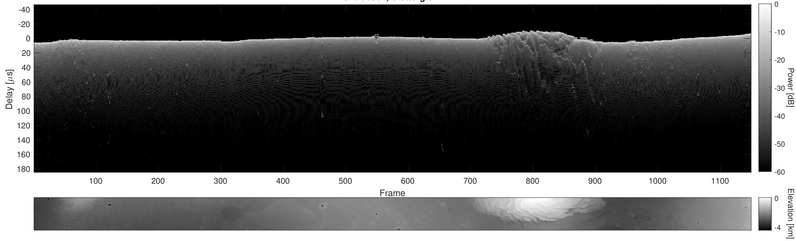
Orbit 9904, Cluttergram
