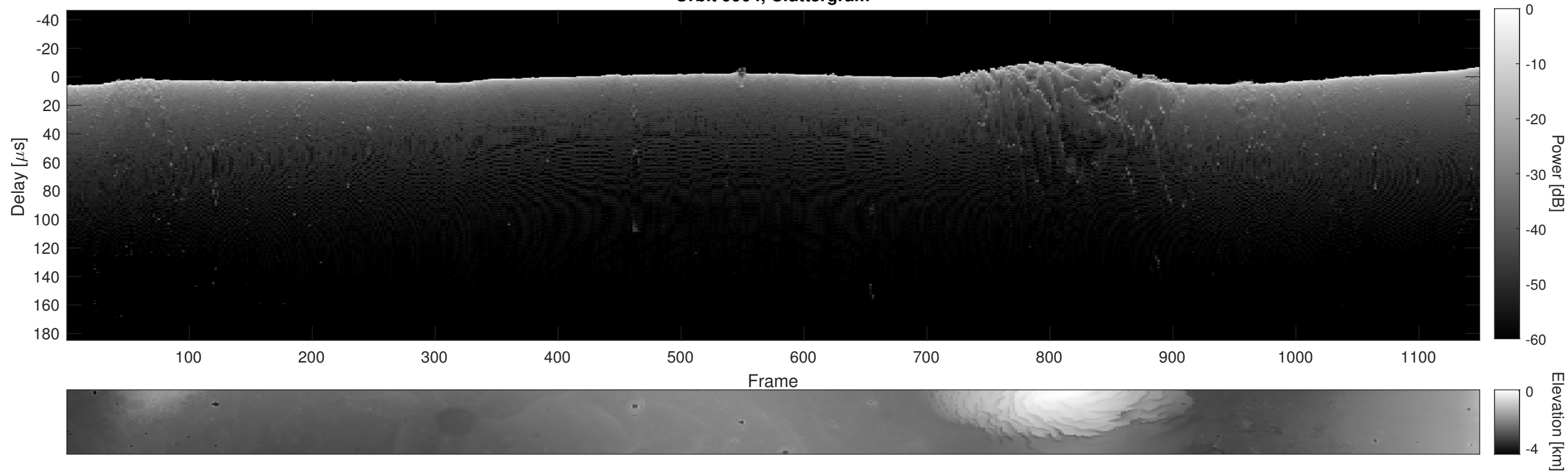
Orbit 9904, Cluttergram
