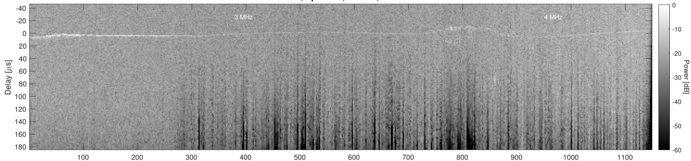
Orbit 9904, Cluttergram
