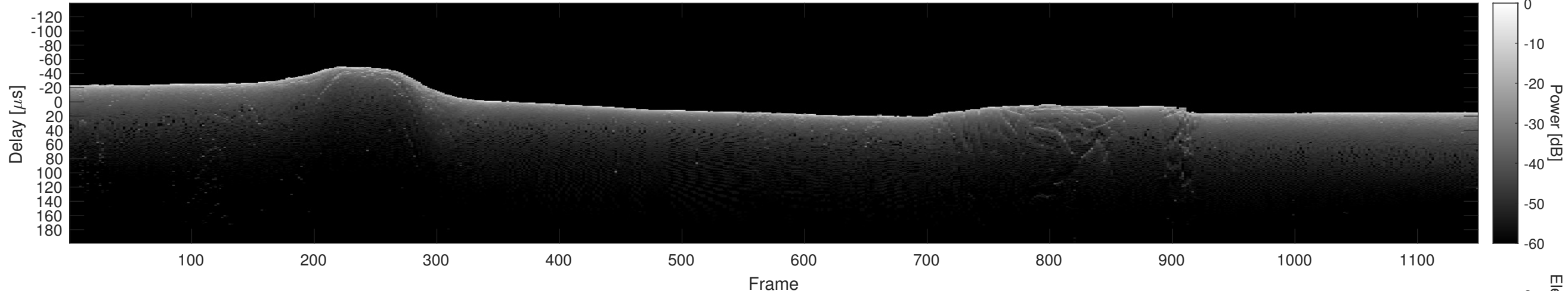
Orbit 9906, Cluttergram
