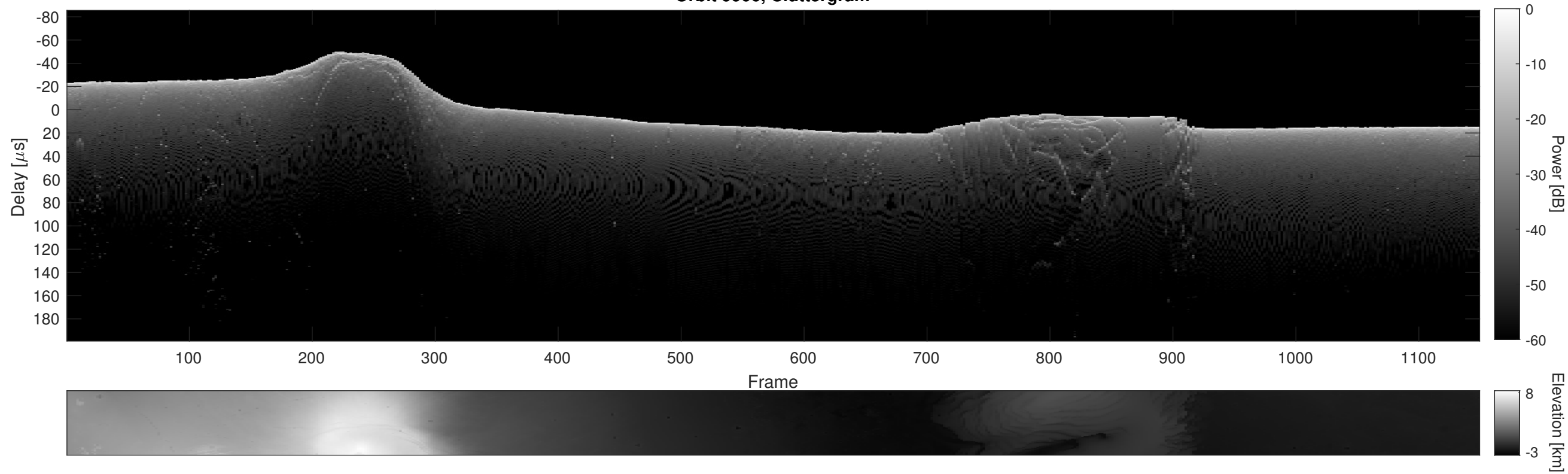
Orbit 9906, Cluttergram
