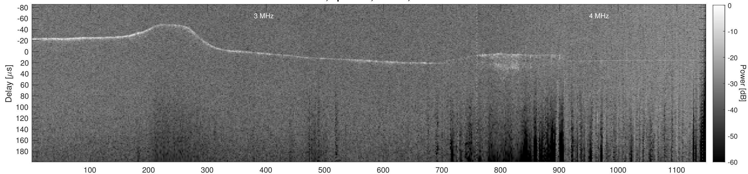
Orbit 9906, Cluttergram
