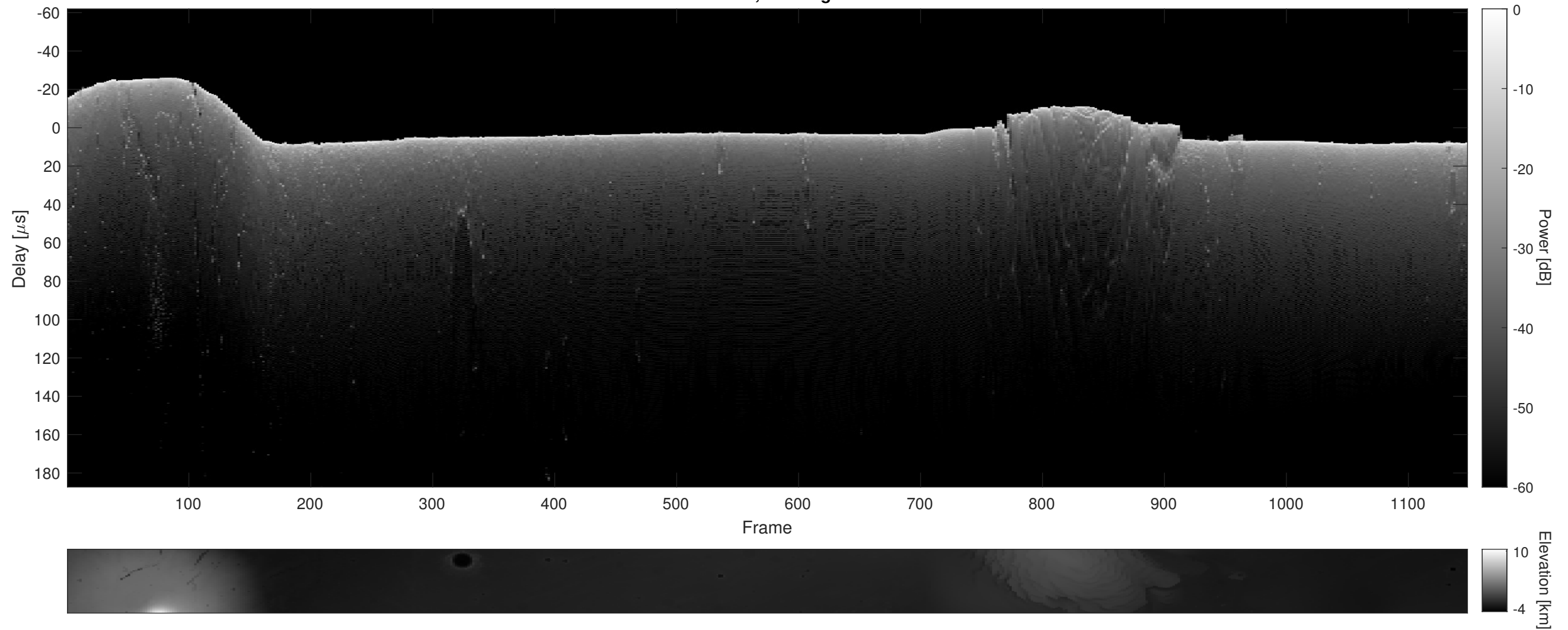
Orbit 9907, Cluttergram
