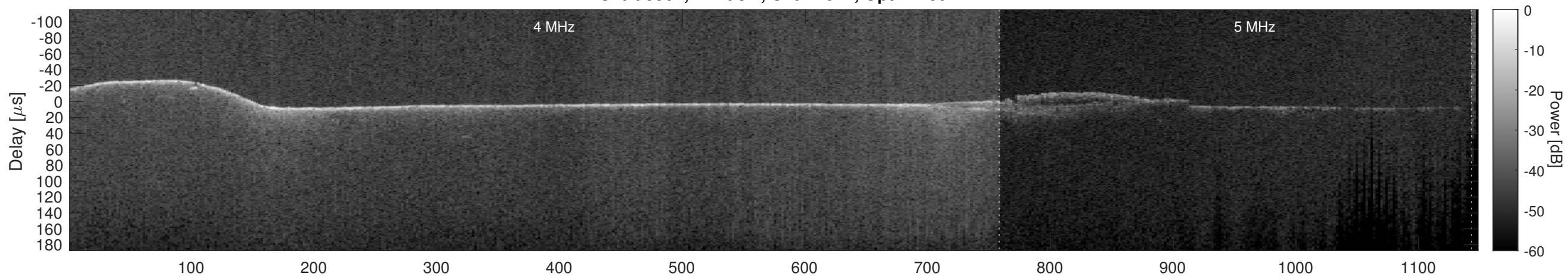
Orbit 9907, Cluttergram
