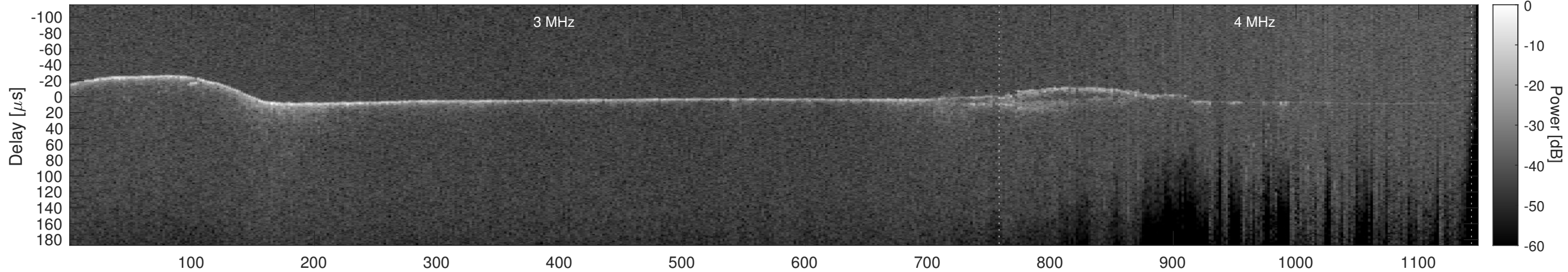
Orbit 9907, Cluttergram
