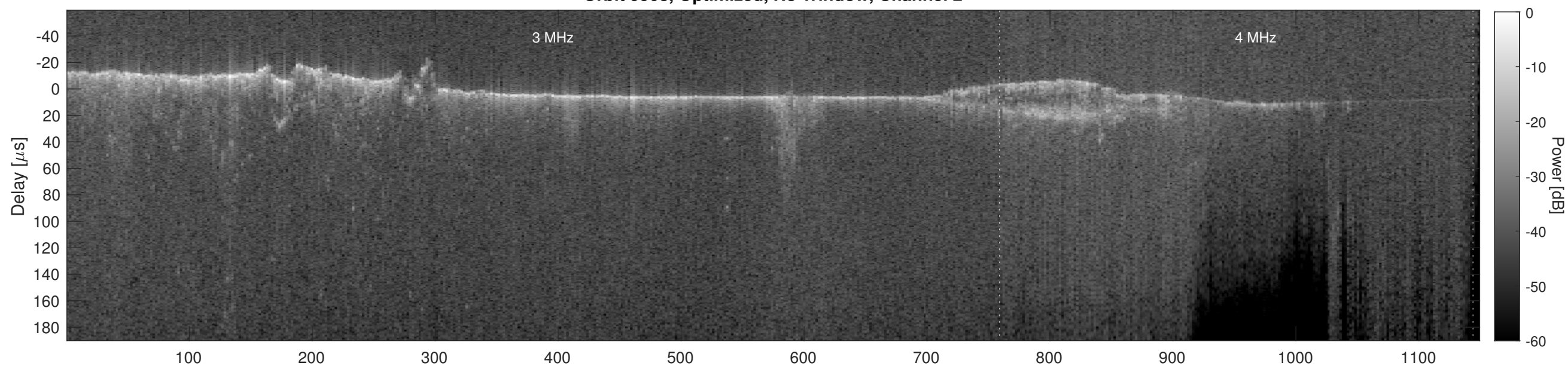
Orbit 9908, Cluttergram
