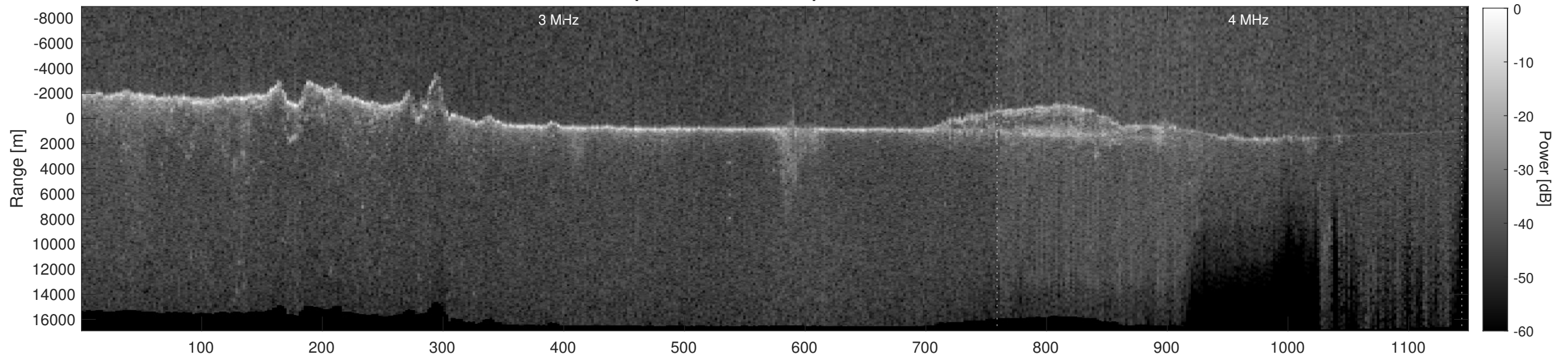
Orbit 9908, Depth-Corrected Cluttergram
