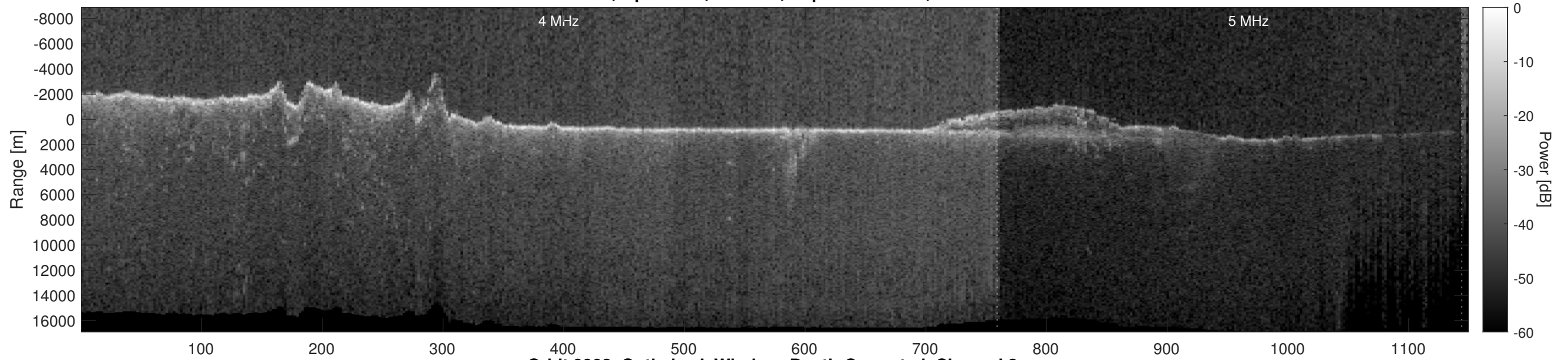
Orbit 9908, Optimized, Window, Depth-Corrected, Channel 2
