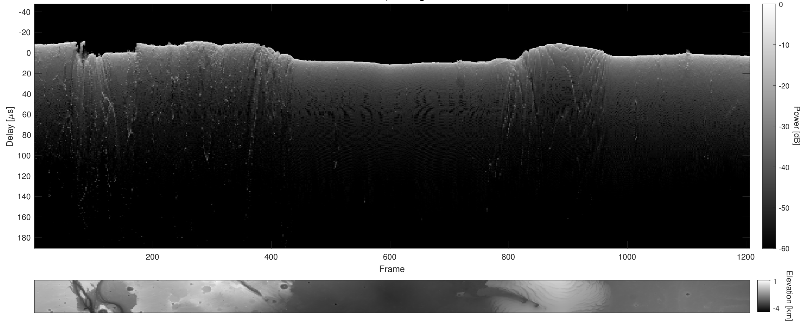
Orbit 9909, Cluttergram
