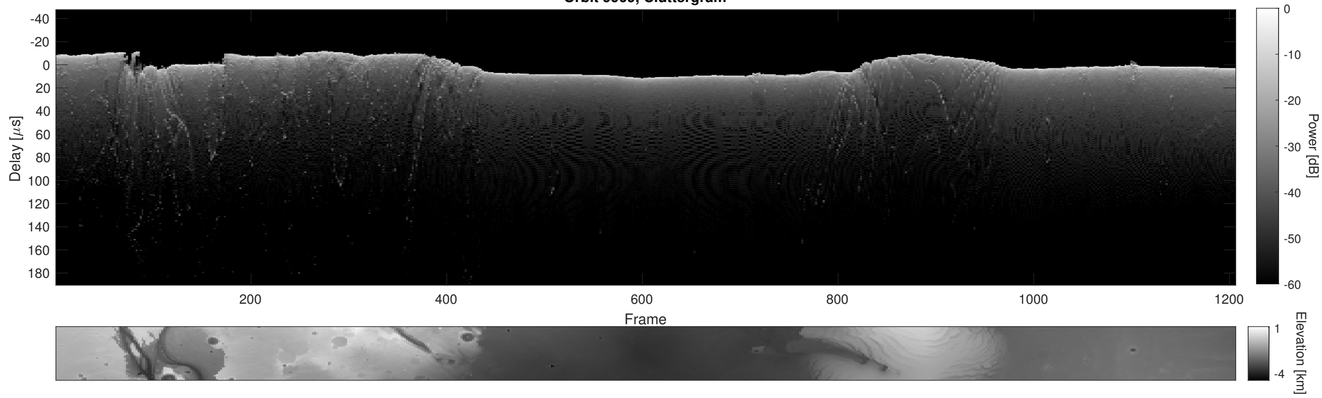
Orbit 9909, Cluttergram
