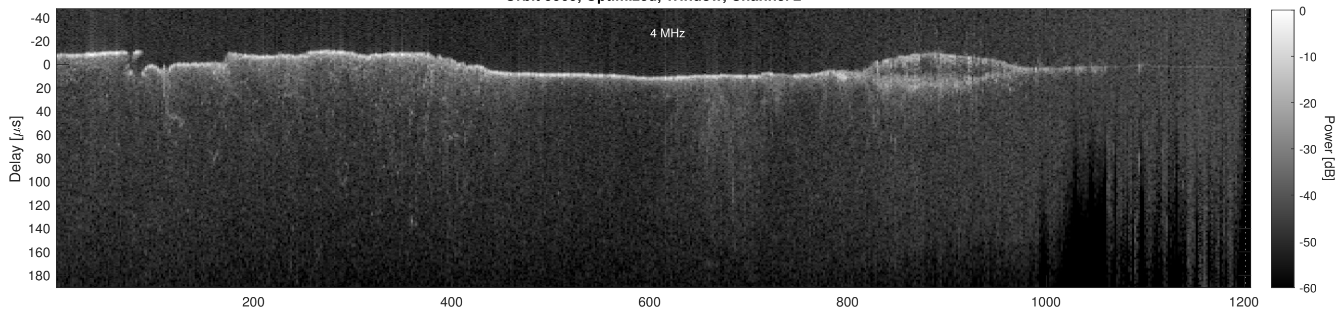
Orbit 9909, Cluttergram
