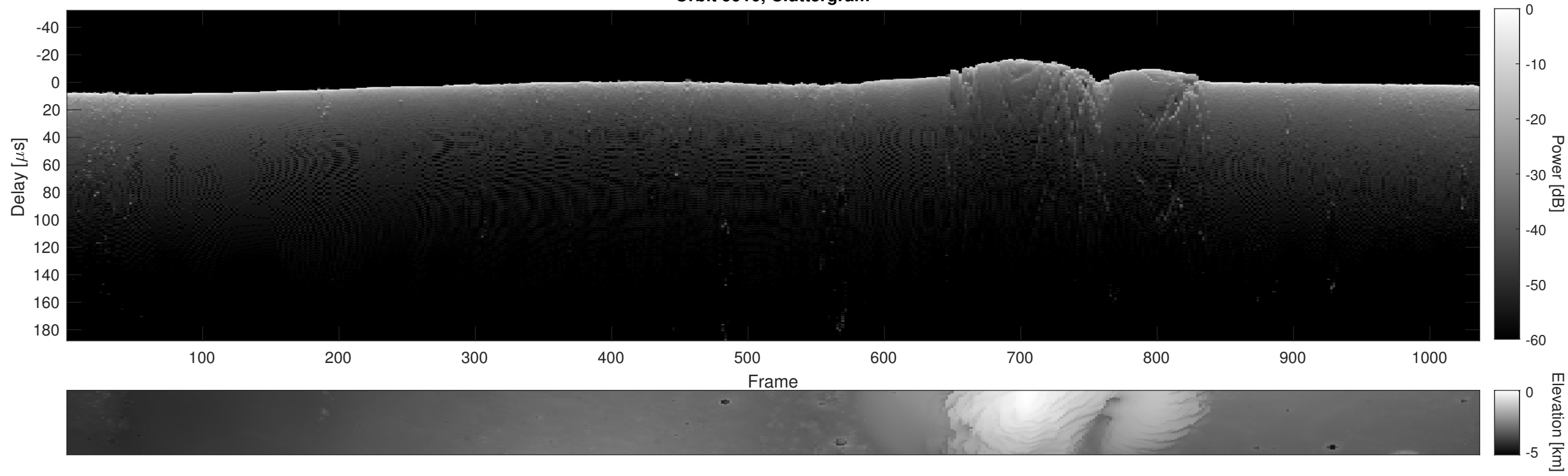
Orbit 9910, Cluttergram
