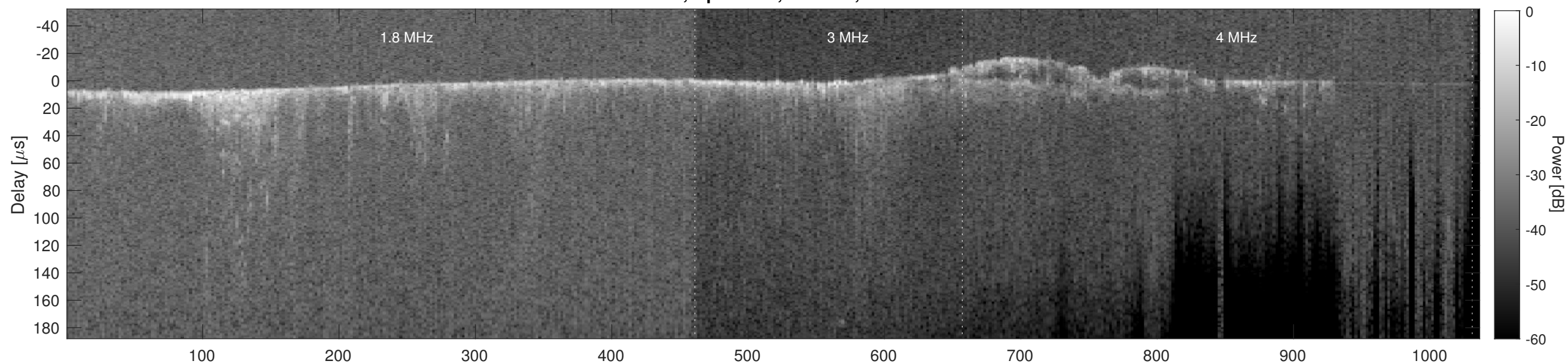
Orbit 9910, Cluttergram
