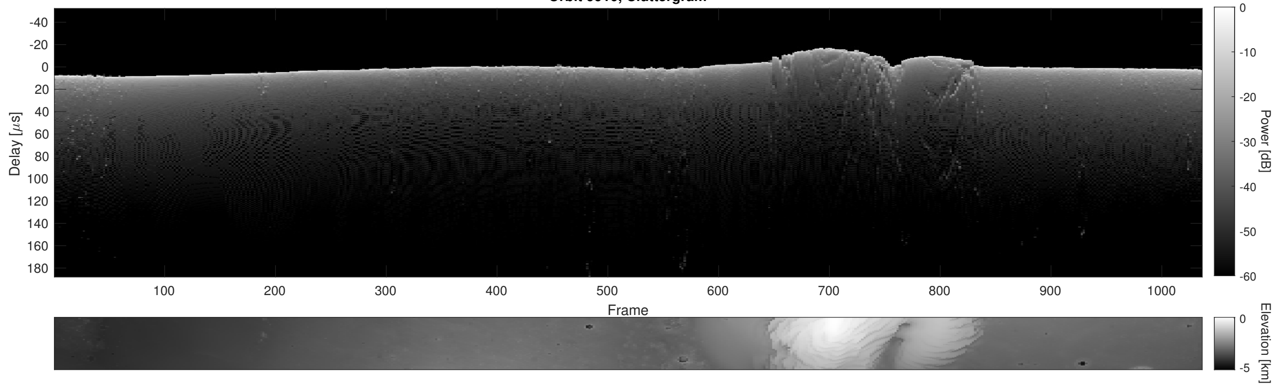
Orbit 9910, Cluttergram
