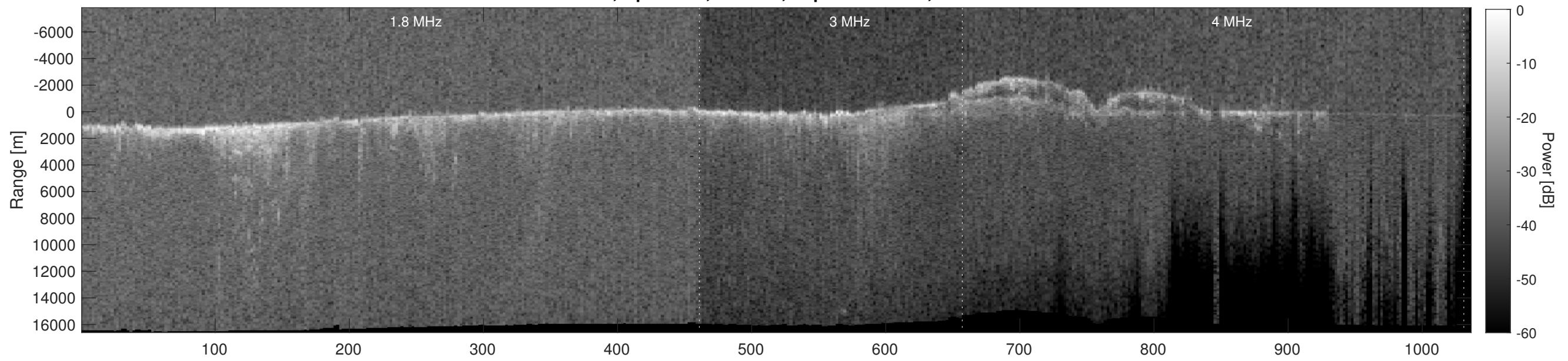
Orbit 9910, Depth-Corrected Cluttergram
