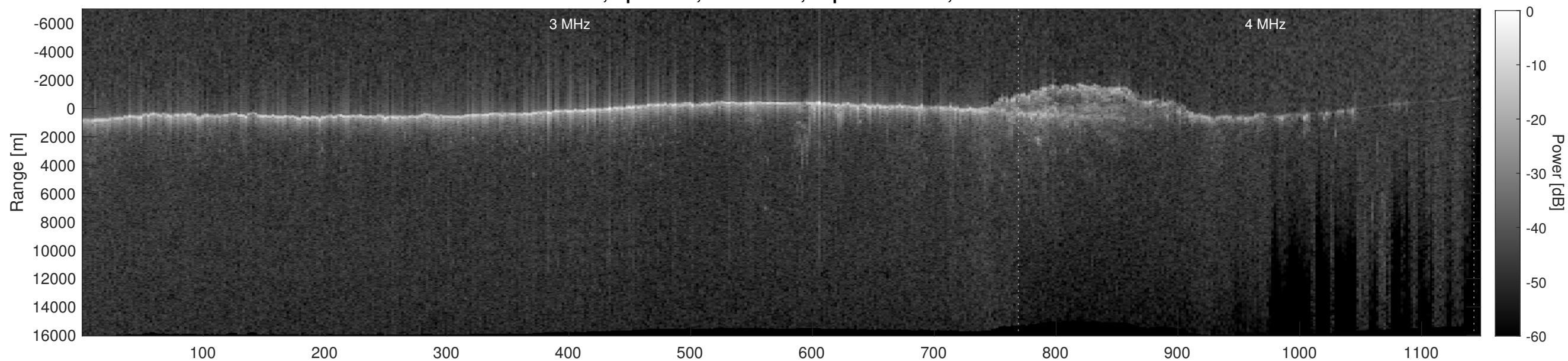
Orbit 9911, Depth-Corrected Cluttergram
