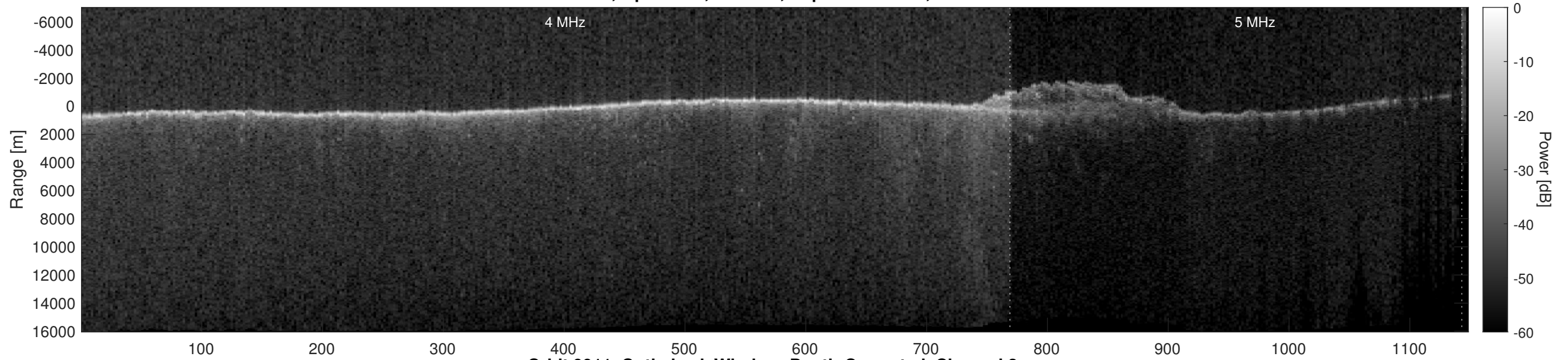
Orbit 9911, Optimized, Window, Depth-Corrected, Channel 2
