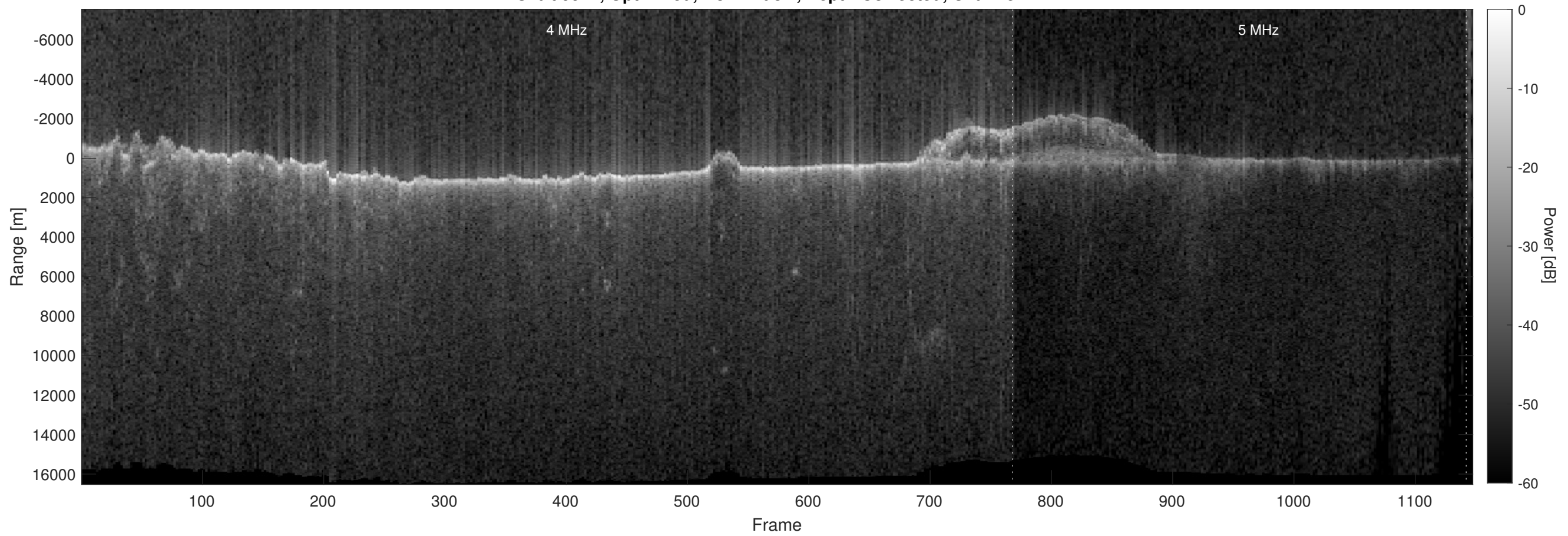
Orbit 9912, Optimized, No Window, Depth-Corrected, Channel 2
