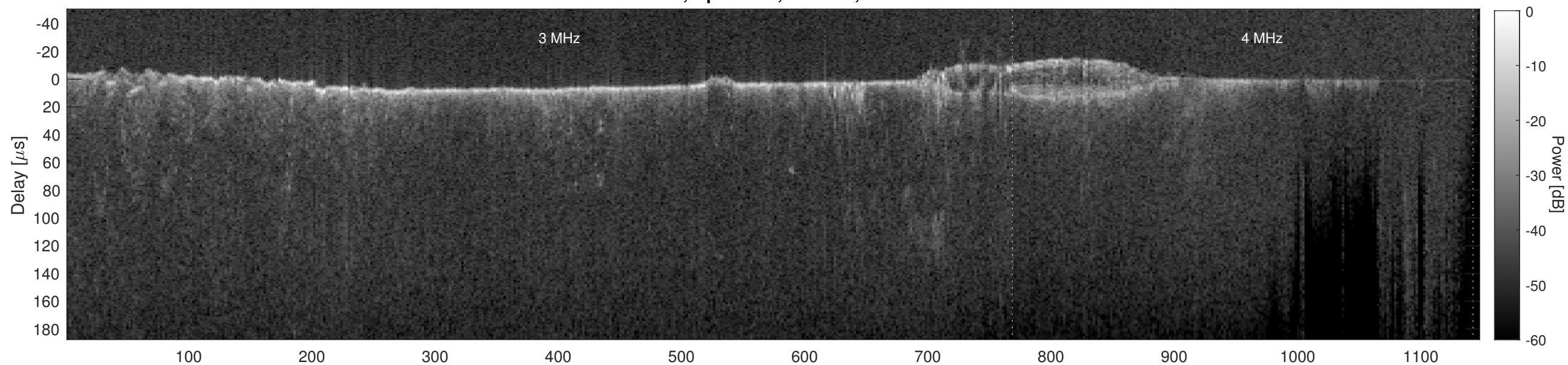
Orbit 9912, Cluttergram
