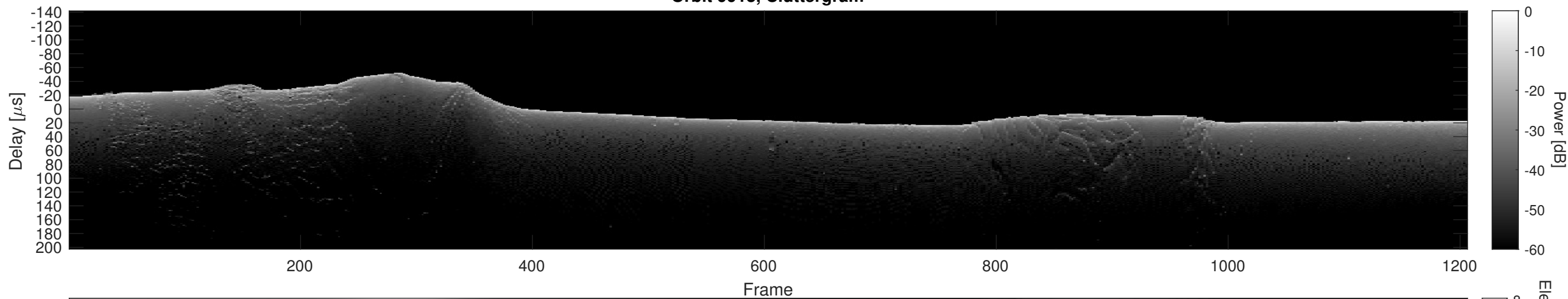
Orbit 9913, Cluttergram
