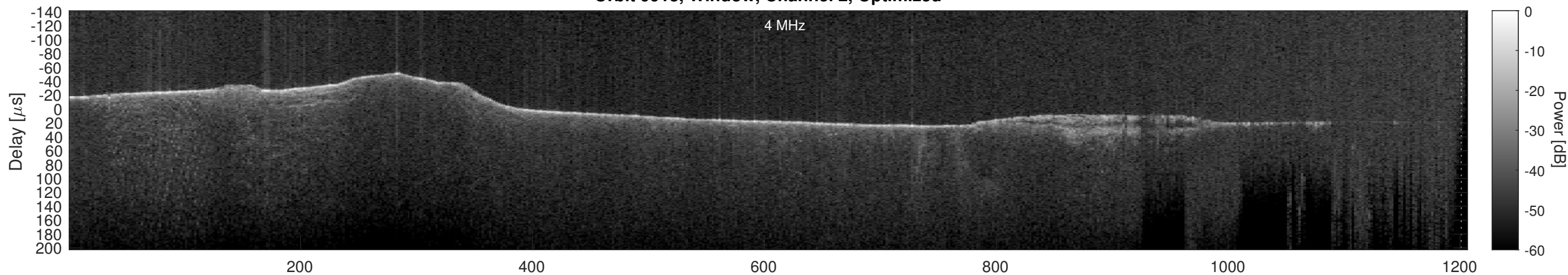
Orbit 9913, Cluttergram
