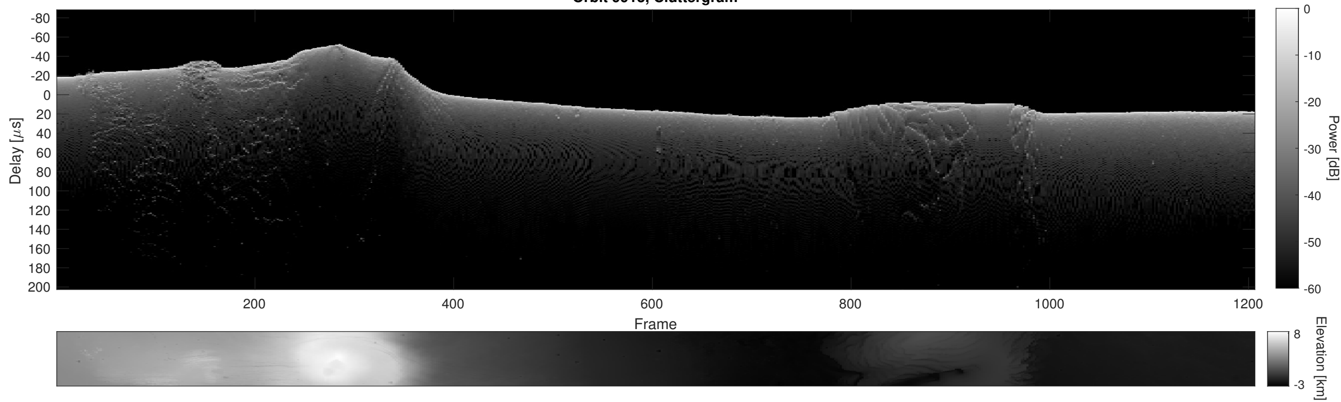
Orbit 9913, Cluttergram
