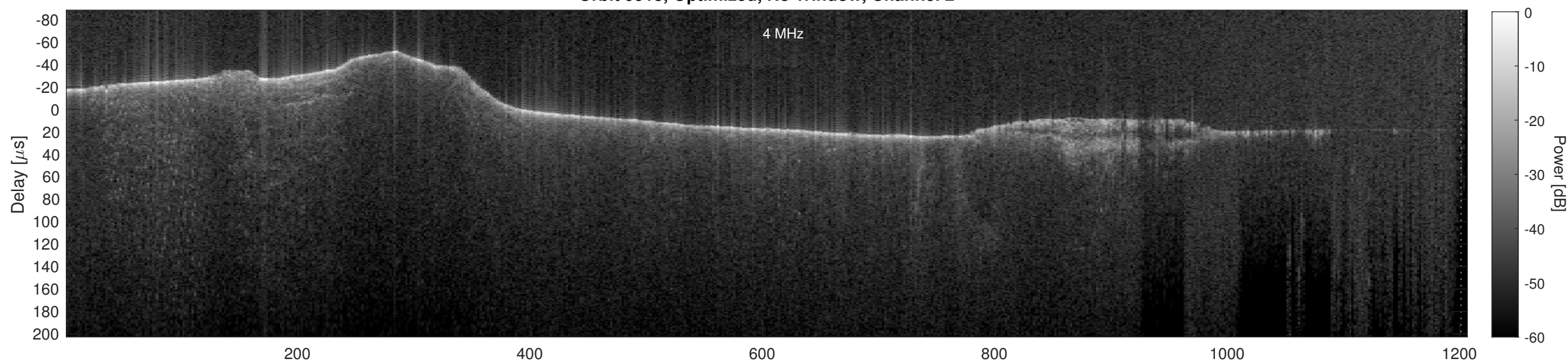
Orbit 9913, Cluttergram
