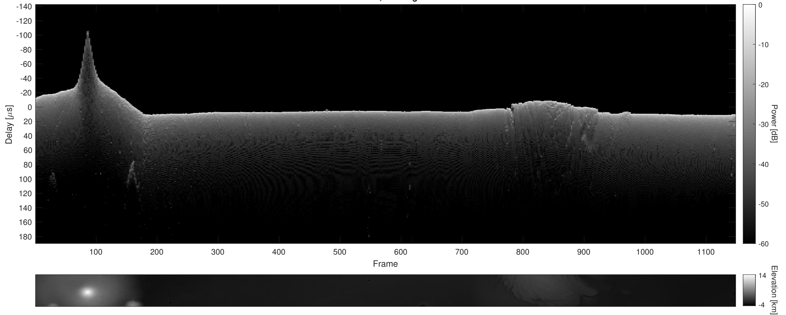
Orbit 9914, Cluttergram
