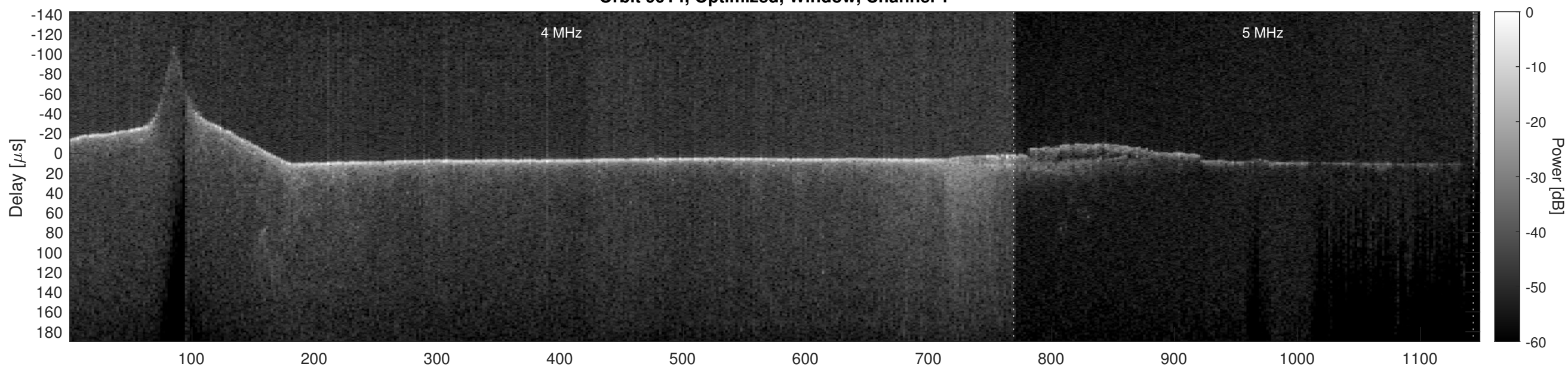
Orbit 9914, Optimized, Window, Channel 2
