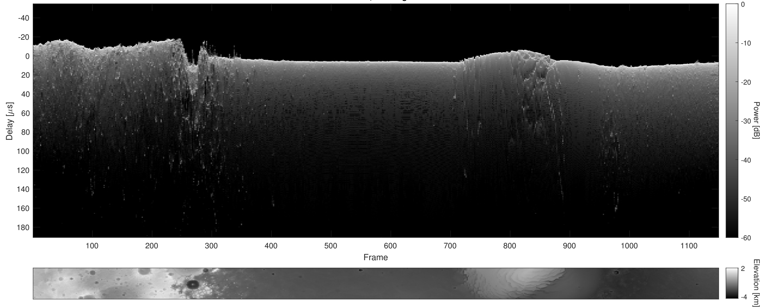
Orbit 9915, Cluttergram
