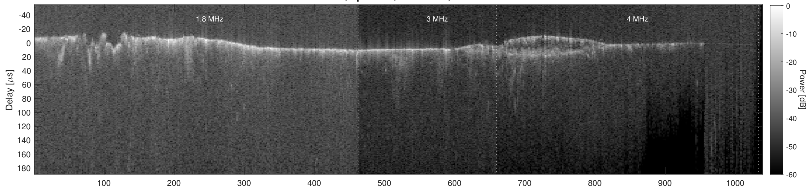
Orbit 9916, Cluttergram
