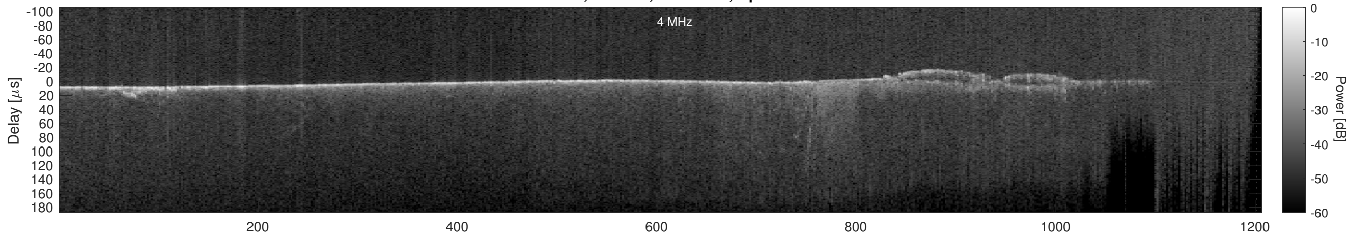
Orbit 9917, Cluttergram
