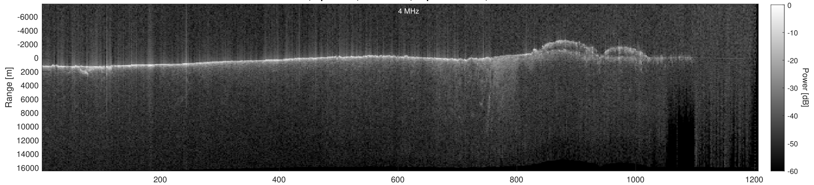
Orbit 9917, Depth-Corrected Cluttergram
