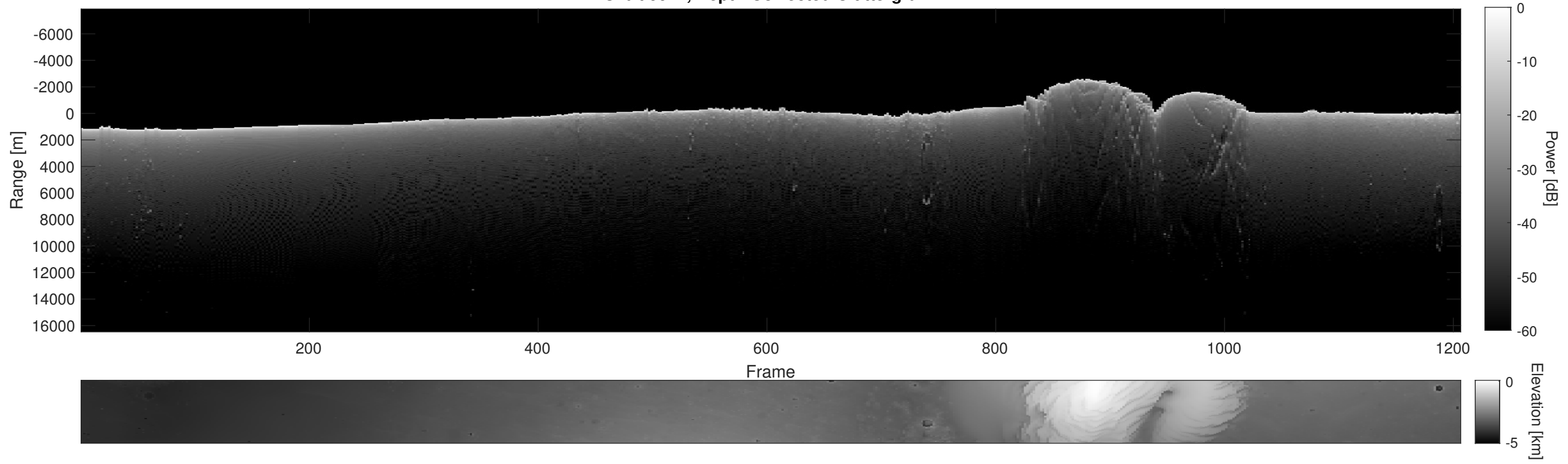
Orbit 9917, Depth-Corrected Cluttergram
