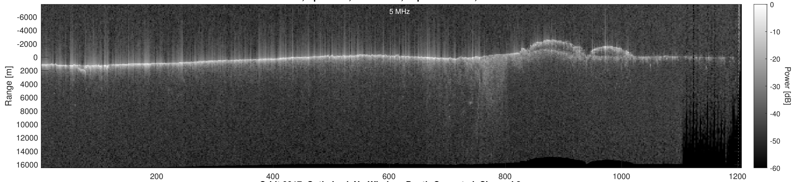
Orbit 9917, Optimized, No Window, Depth-Corrected, Channel 2
