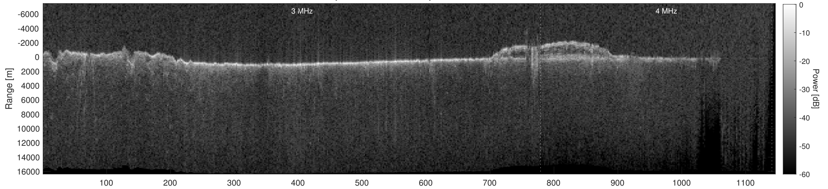
Orbit 9919, Depth-Corrected Cluttergram
