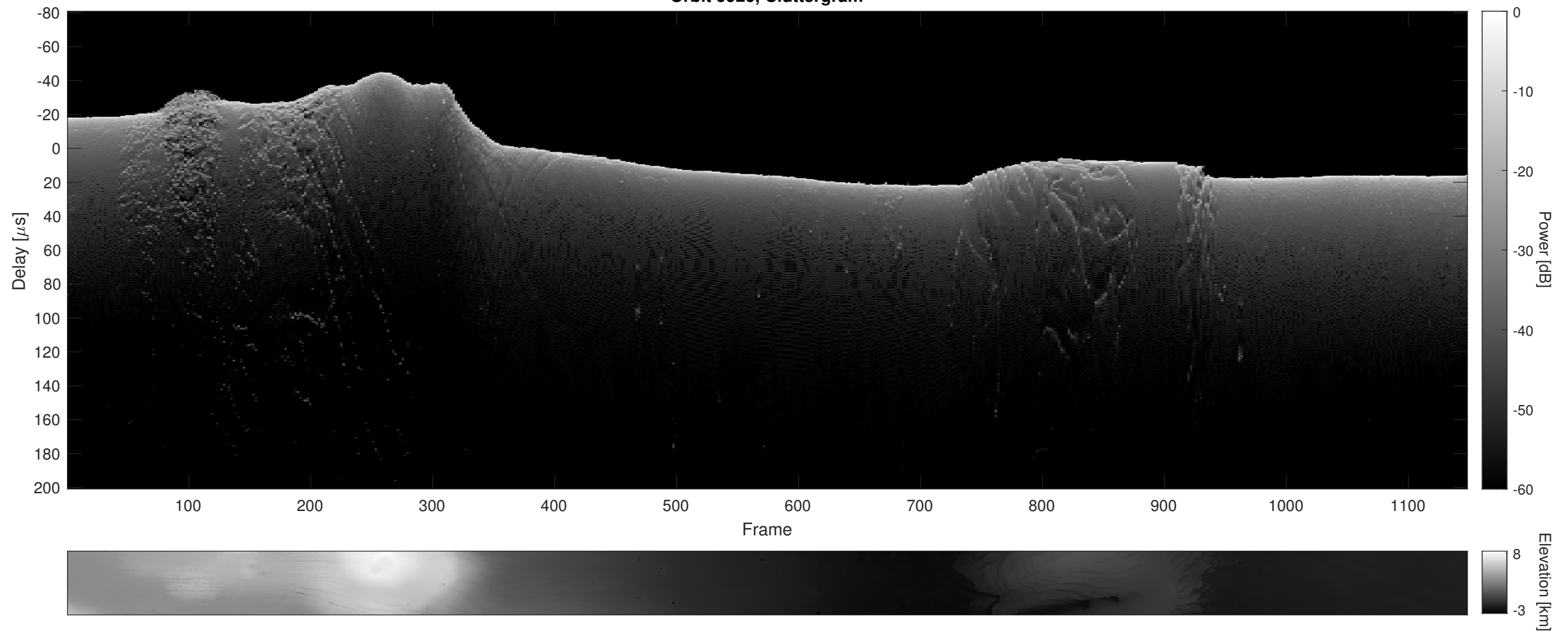
Orbit 9920, Cluttergram
