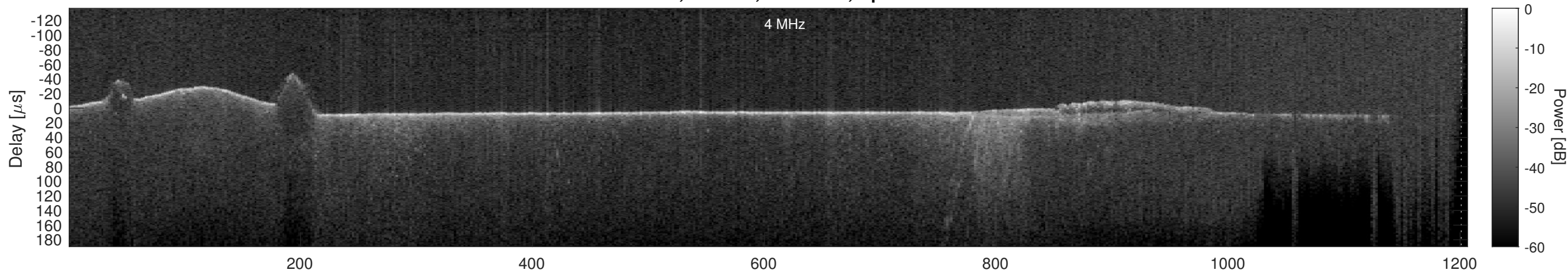
Orbit 9921, Cluttergram
