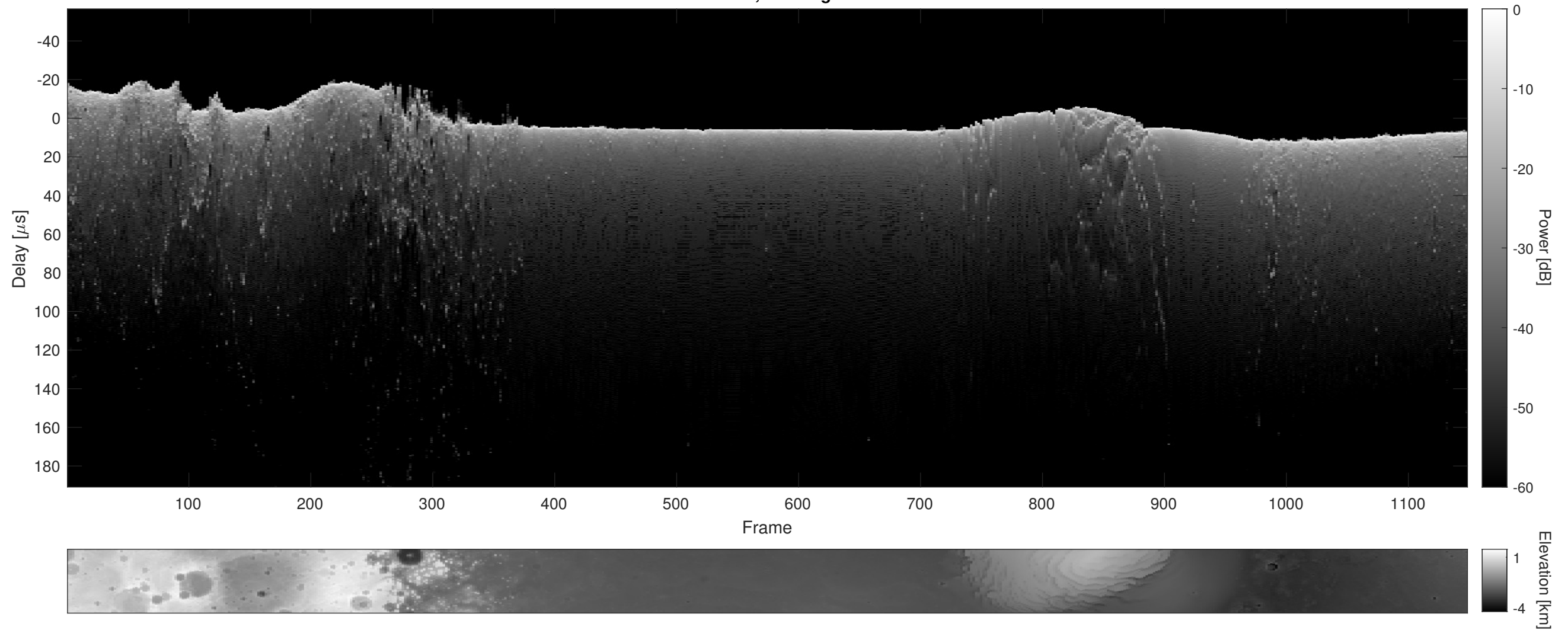
Orbit 9922, Cluttergram
