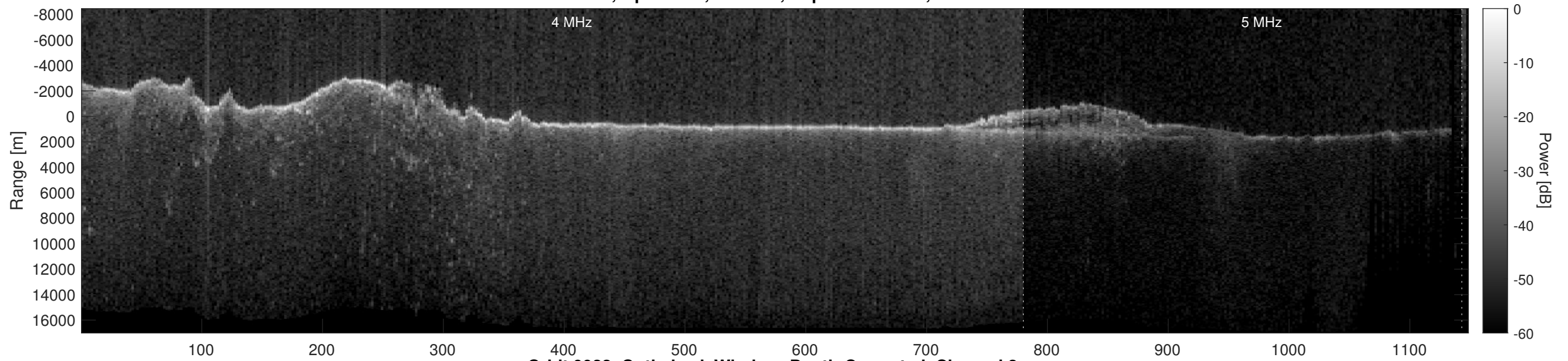
Orbit 9922, Optimized, Window, Depth-Corrected, Channel 2
