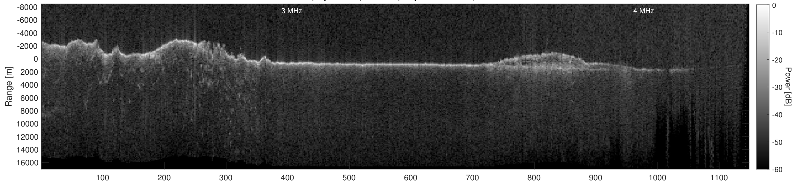
Orbit 9922, Depth-Corrected Cluttergram
