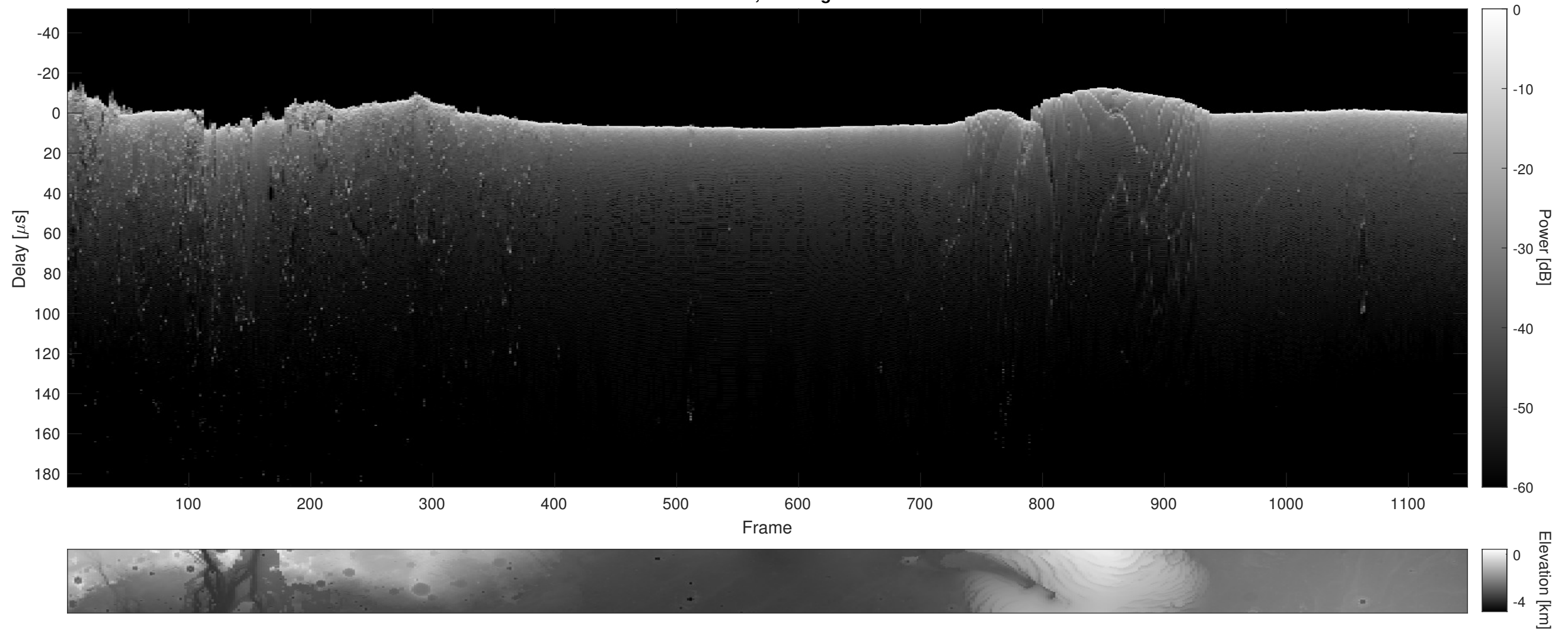
Orbit 9923, Cluttergram
