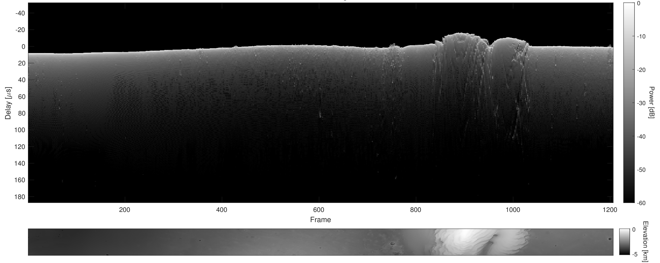
Orbit 9924, Cluttergram
