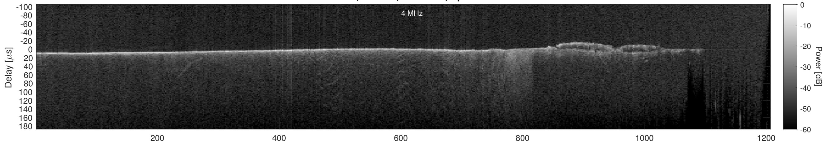
Orbit 9924, Cluttergram
