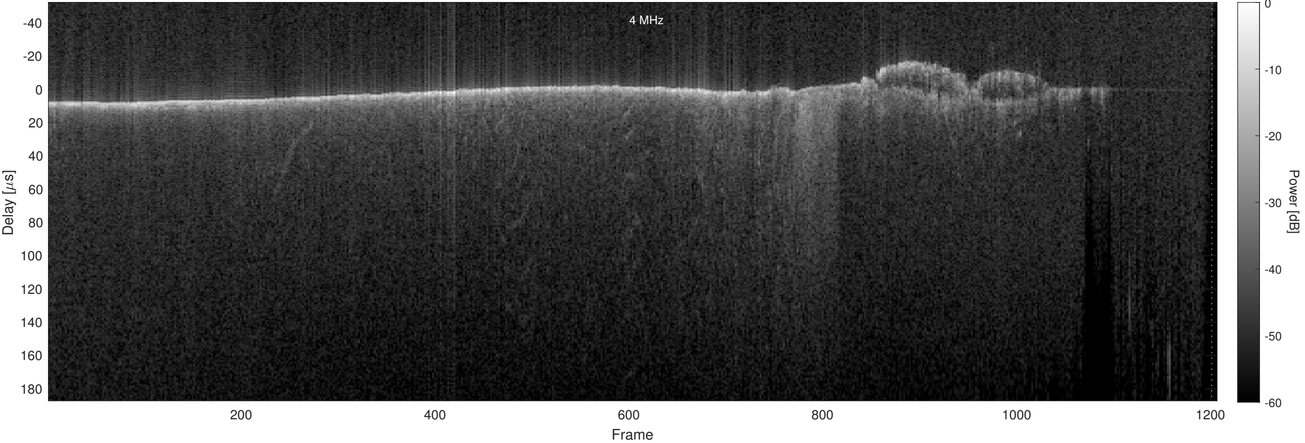
Orbit 9924, Optimized, No Window, Channel 2
