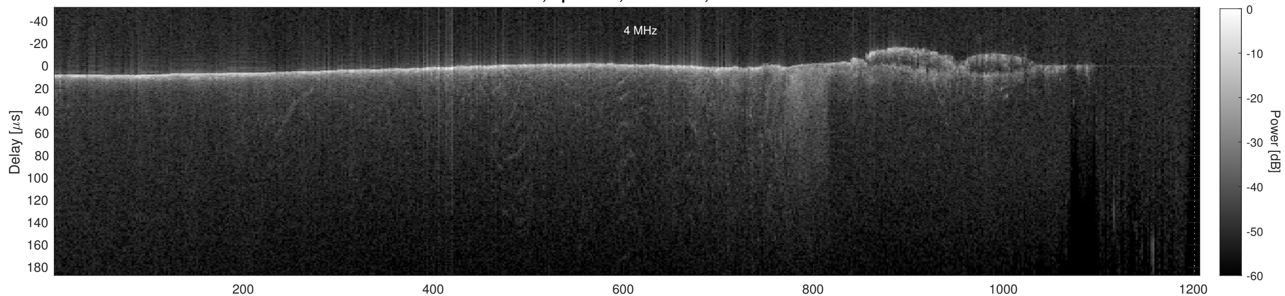
Orbit 9924, Cluttergram
