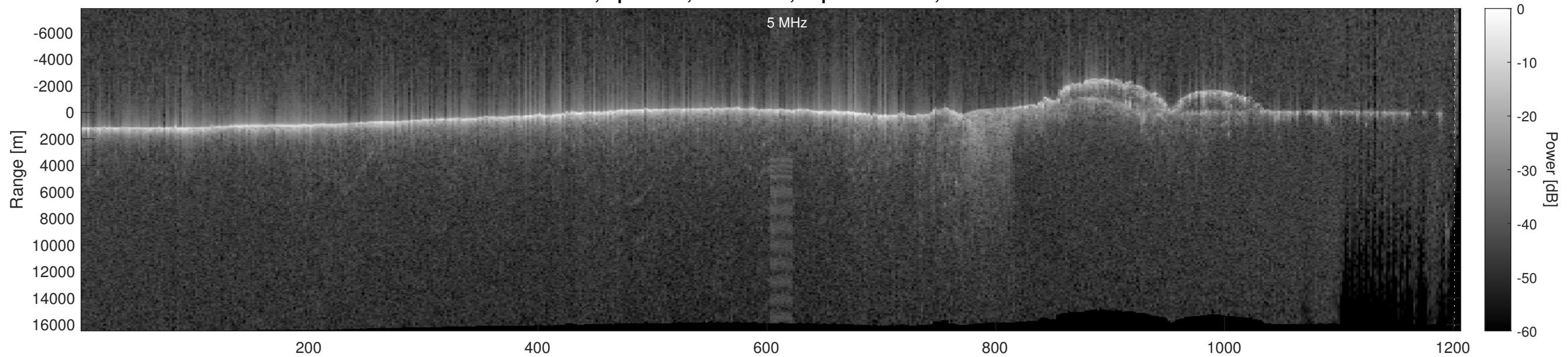
Orbit 9924, Optimized, No Window, Depth-Corrected, Channel 2
