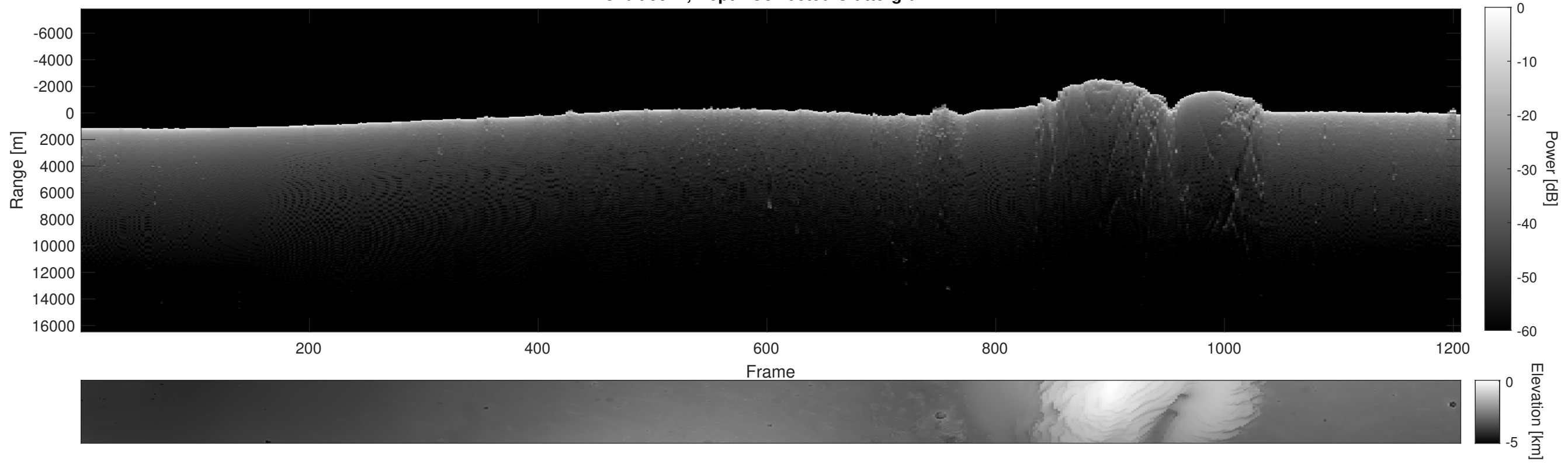
Orbit 9924, Depth-Corrected Cluttergram
