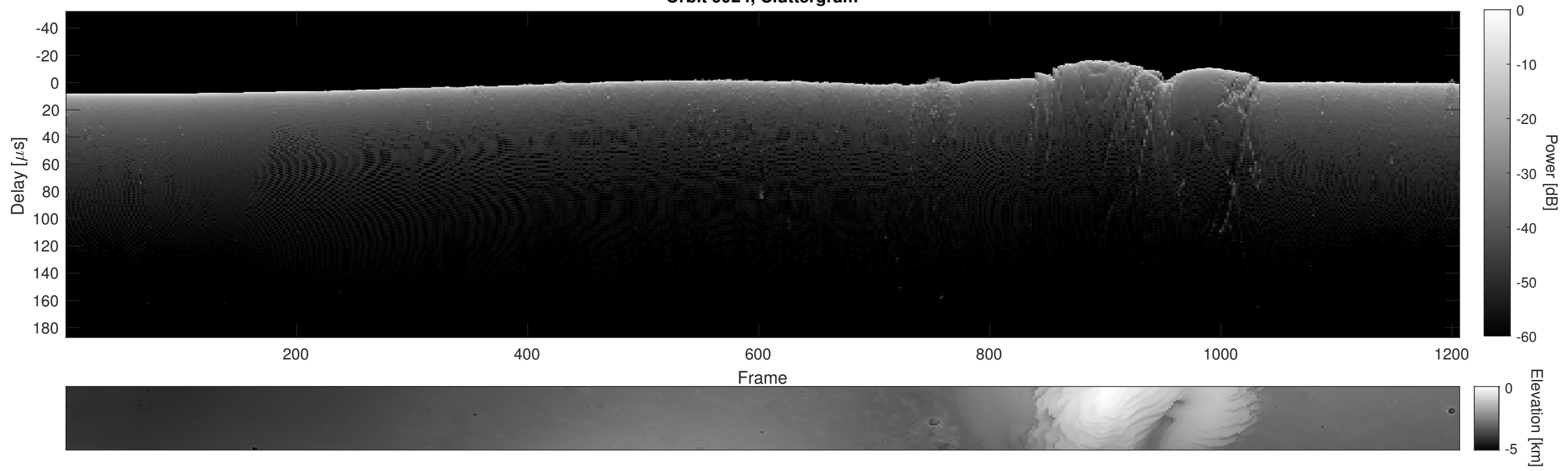
Orbit 9924, Cluttergram
