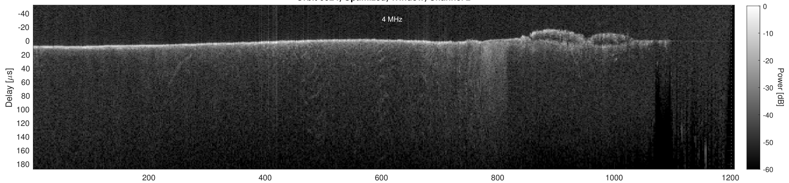
Orbit 9924, Cluttergram
