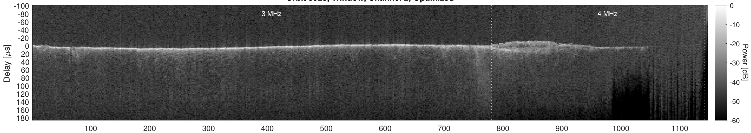
Orbit 9925, Cluttergram
