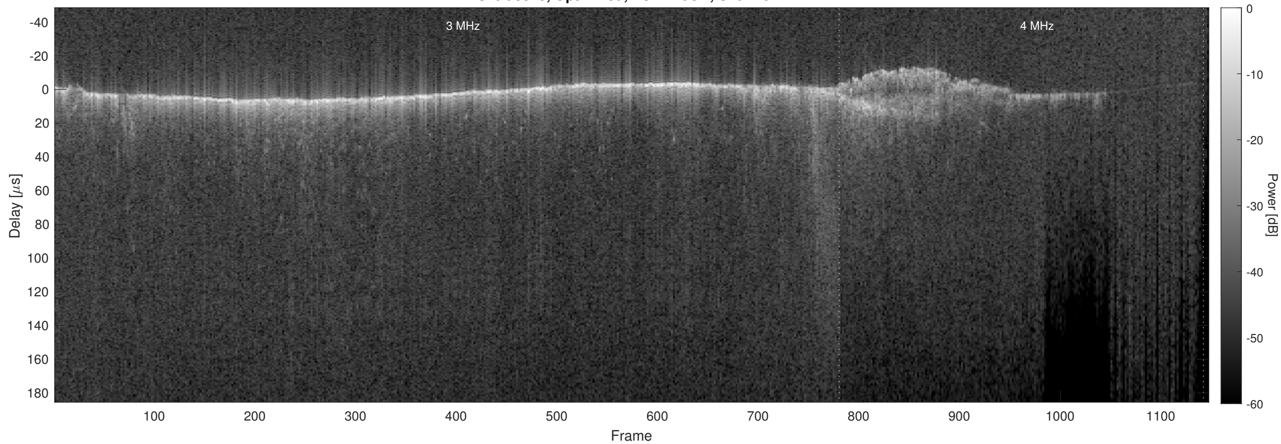
Orbit 9925, Optimized, No Window, Channel 2
