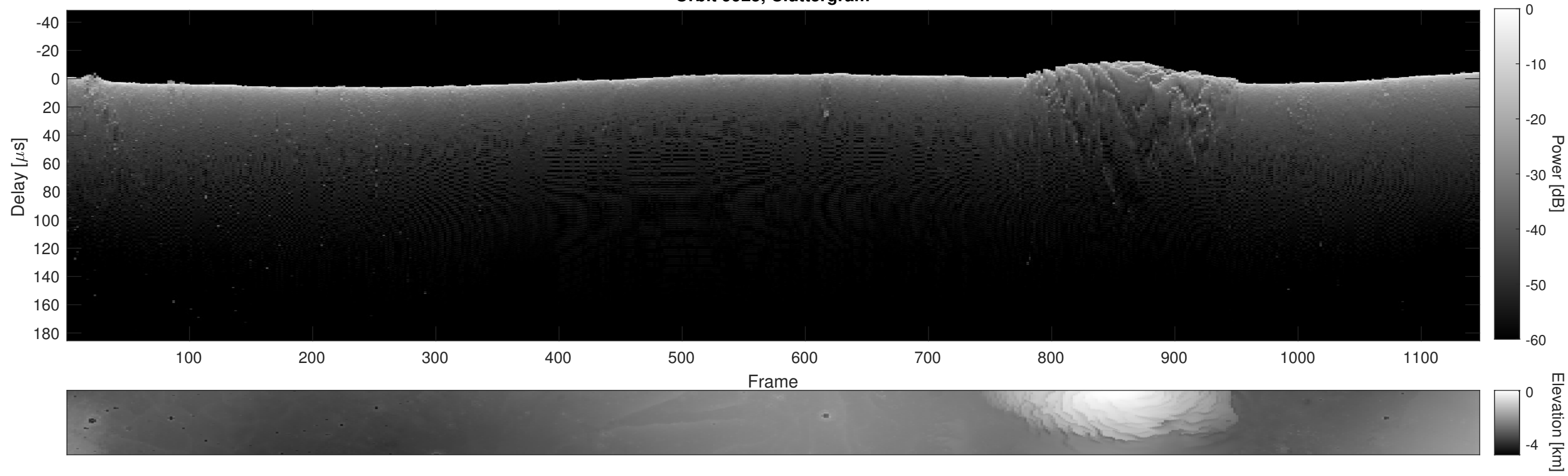
Orbit 9925, Cluttergram
