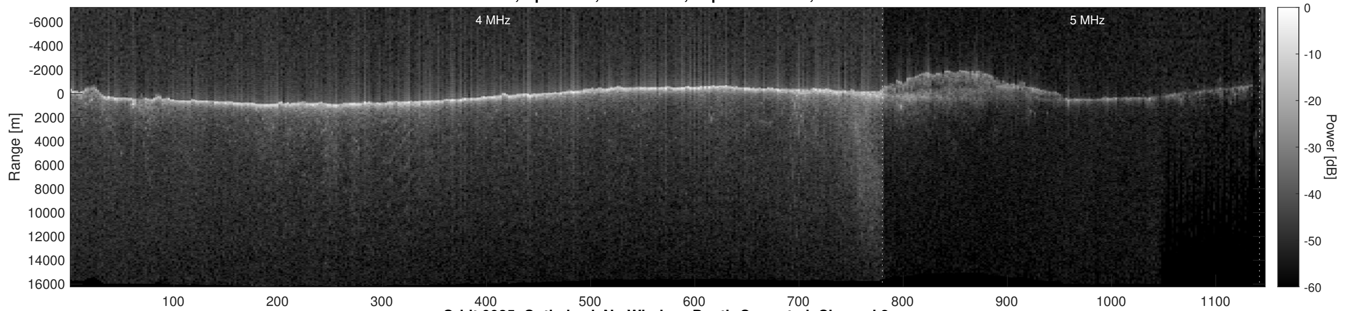
Orbit 9925, Optimized, No Window, Depth-Corrected, Channel 2
