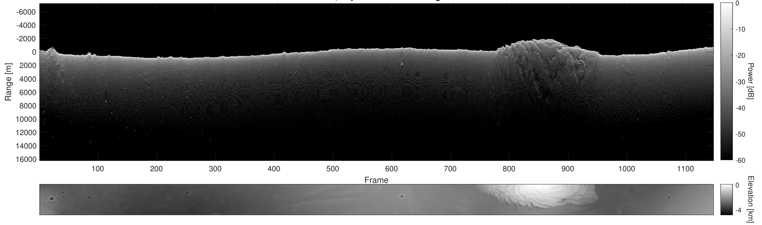
Orbit 9925, Depth-Corrected Cluttergram
