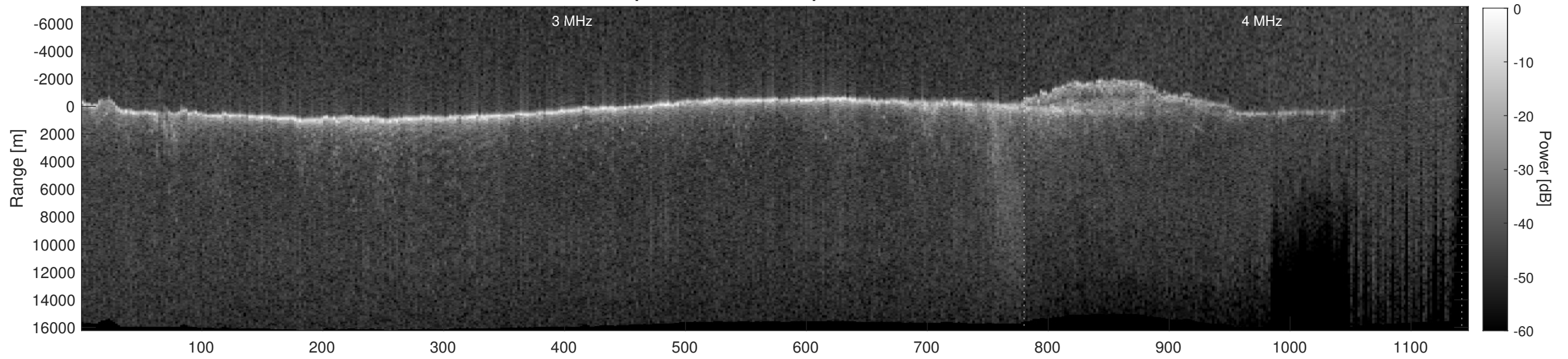
Orbit 9925, Depth-Corrected Cluttergram
