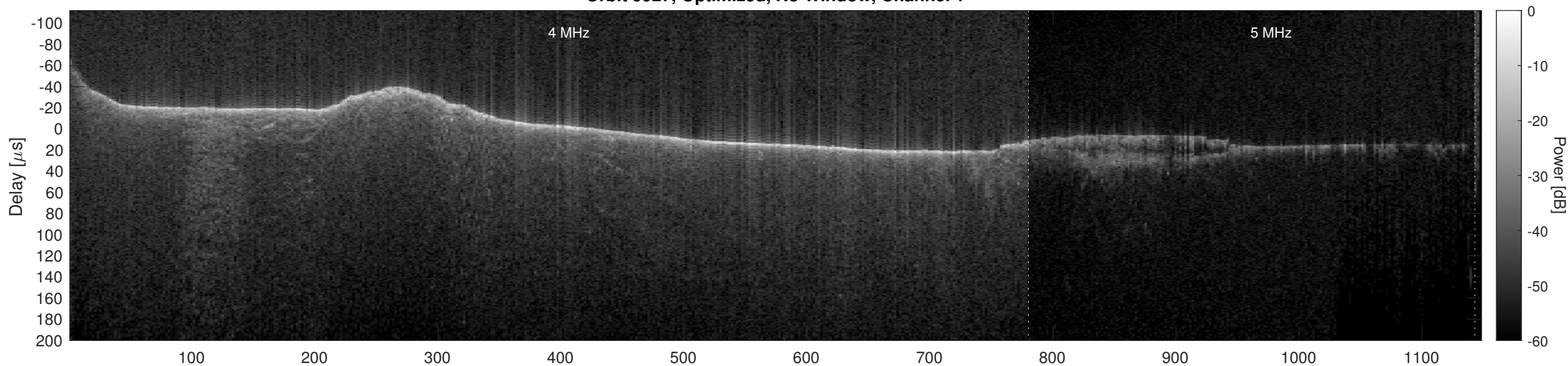
Orbit 9927, Optimized, No Window, Channel 2
