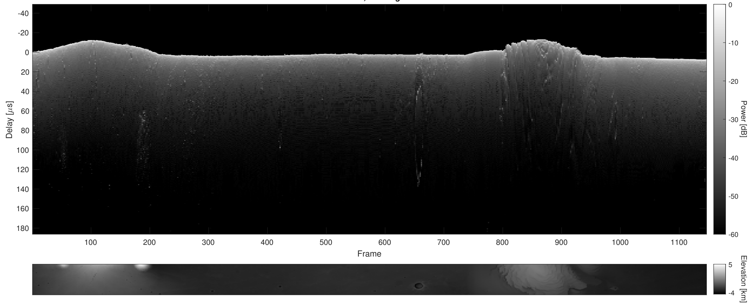
Orbit 9928, Cluttergram
