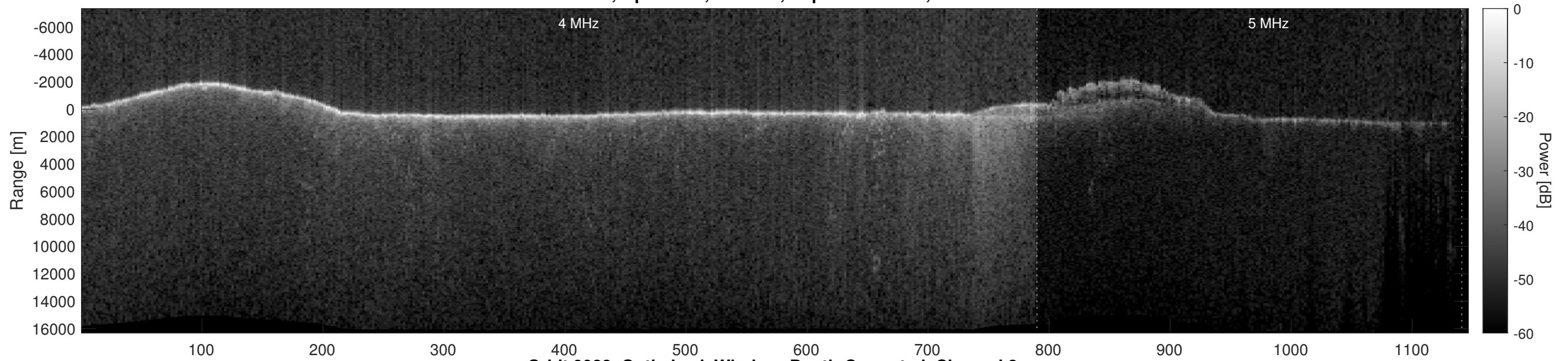
Orbit 9928, Optimized, Window, Depth-Corrected, Channel 2
