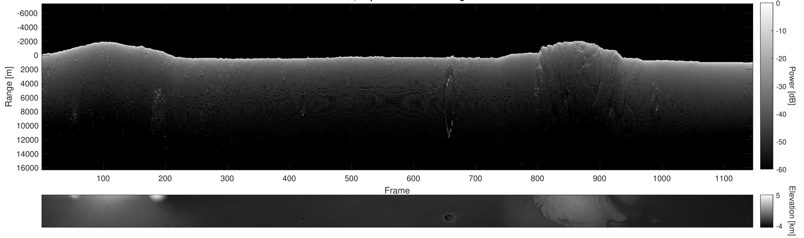
Orbit 9928, Depth-Corrected Cluttergram
