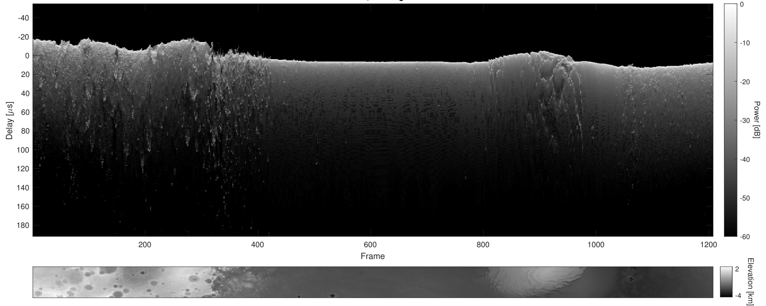
Orbit 9929, Cluttergram
